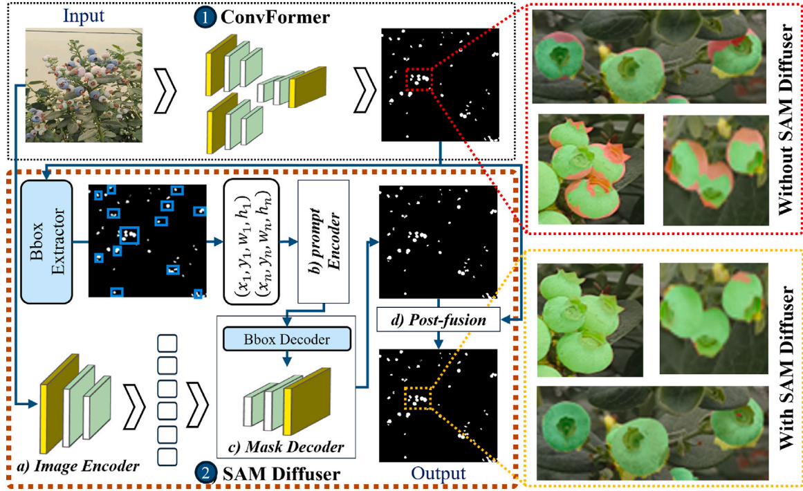
Fig. 4. Architectural overview of the SAM diffuser (with some comparative visual output results) integrated as a secondary refinement stage to improve segmentation accuracy by addressing challenges such as overlapping clusters, blurred regions, and occluded structures.
