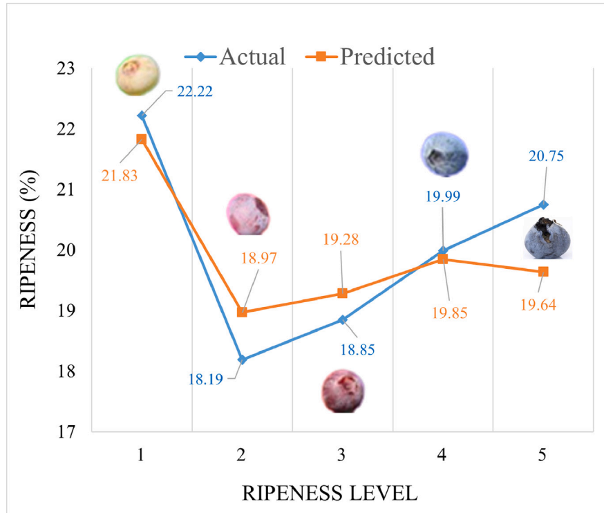
Fig. 9. Illustration of average ripeness distribution P_{r,avg} across five maturity levels ( r_1 to r_5 ), comparing predicted ripeness with ground-truth segmentation results using the same estimation algorithm.
