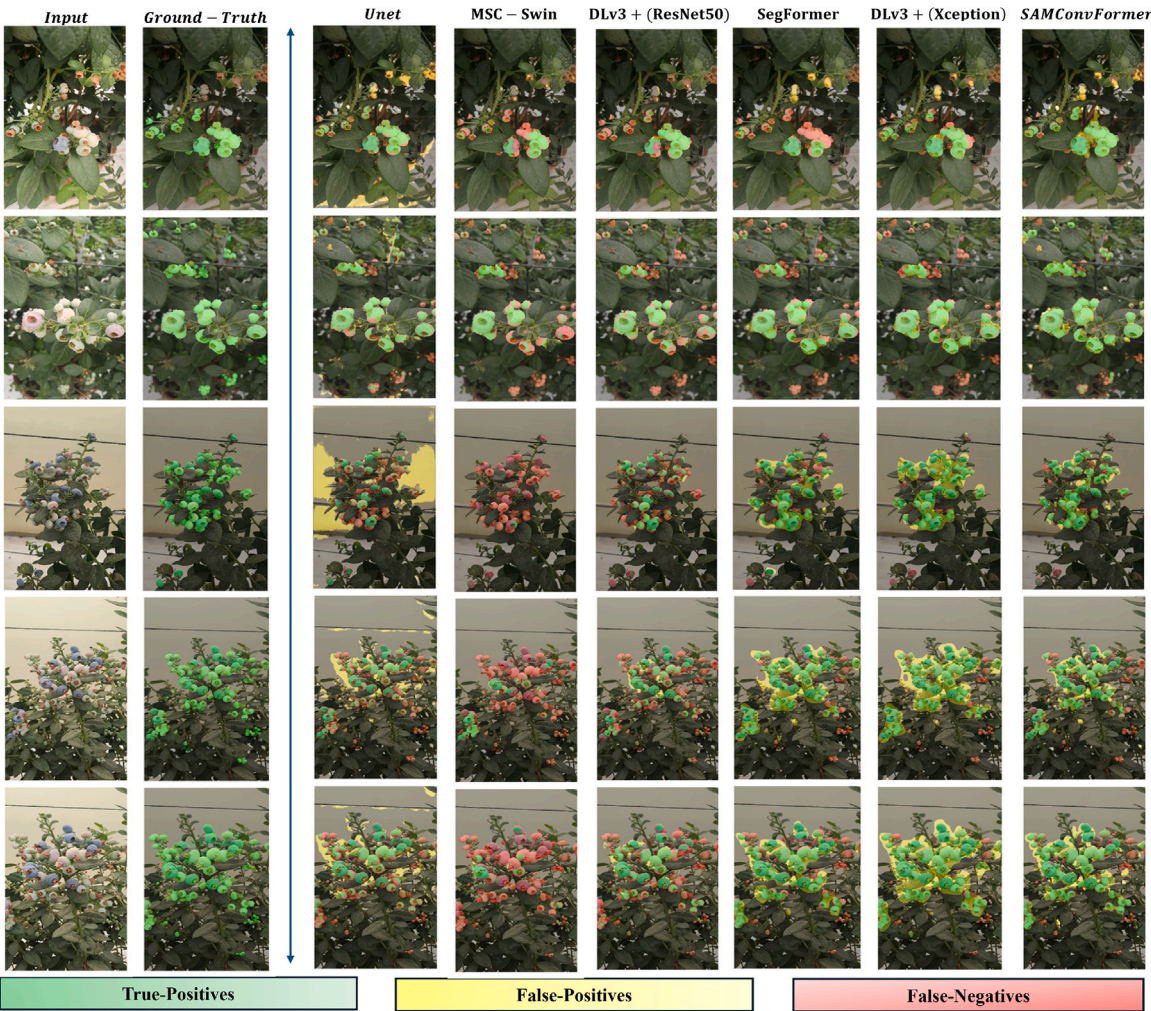
Fig. 10. Qualitative comparison of the proposed SAMConvFormer model with state-of-the-art methods for crop segmentation. The first column shows input images and corresponding ground-truth overlays, while subsequent columns display segmentation results.
