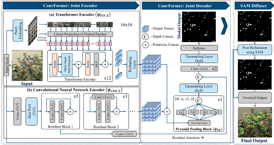
Fig. 3. Architectural overview of the proposed SAMConvFormer framework, which comprises three segments: 1) joint encoder, 2) joint decoder, and 3) SAM diffuser, enabling precise segmentation in complex and real-world agricultural scenarios.
