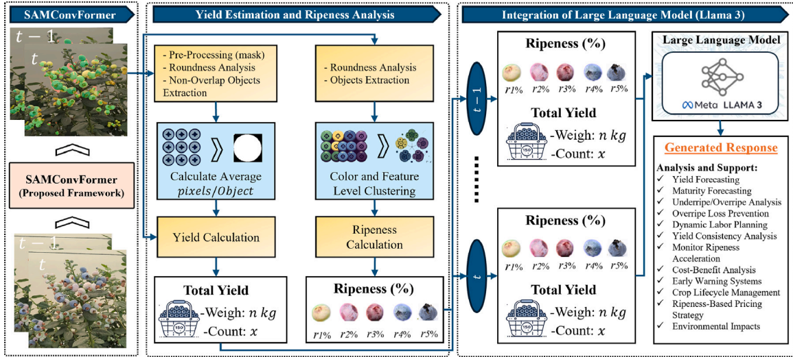
Fig. 2. Workflow of the proposed framework, comprising fruit segmentation with SAMConvFormer, yield estimation and ripeness analysis via a statistical algorithm, and actionable crop management through LLM integration.
